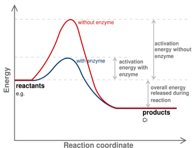
Figure 2: Energy diagram of a reaction in the presence and absence of enzyme
